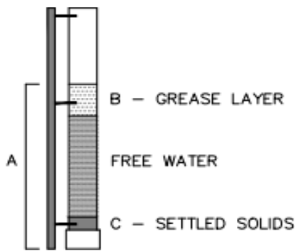
MEASURING DEVICE NTS
