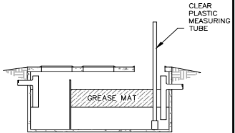
MEASURING TECHNIQUE NTS
